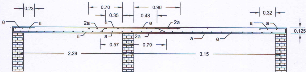
Section 3-3
