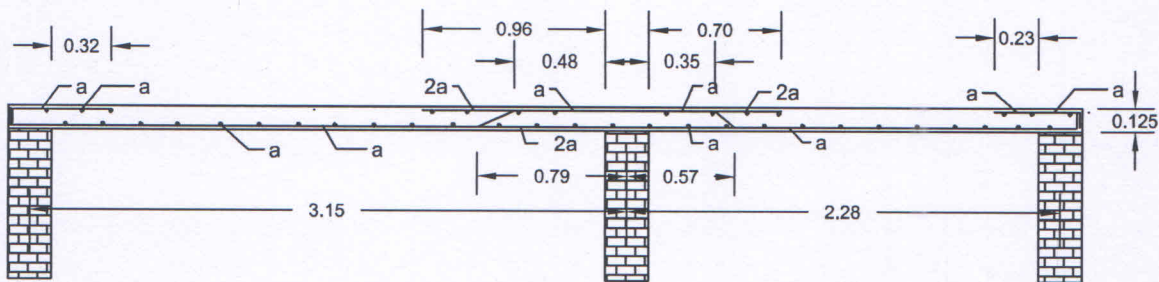
Section 4-4
