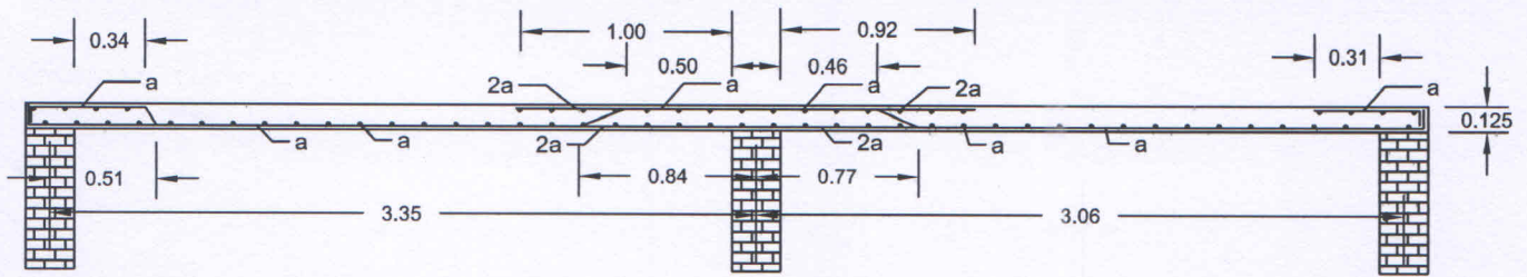
Section 1-1
