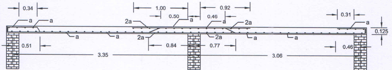
Section 2-2
