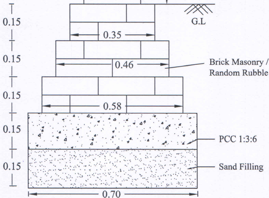
FOOTING DETAILS
